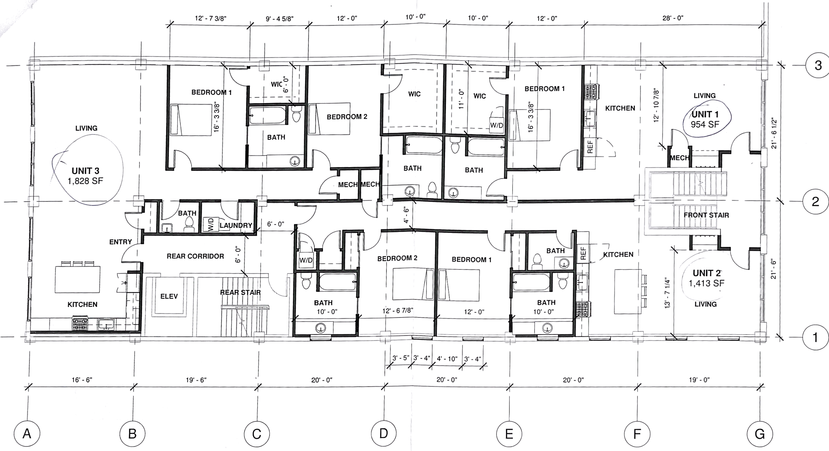
SECOND LEVEL FLOOR PLAN 1/8" = 1'-0"
