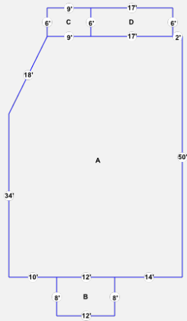
Building Sketch
