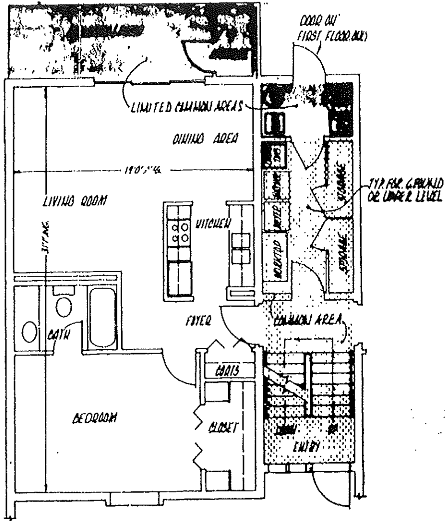
UNIT A - 1 BEDROOM (LEFT) 590 S.F.
